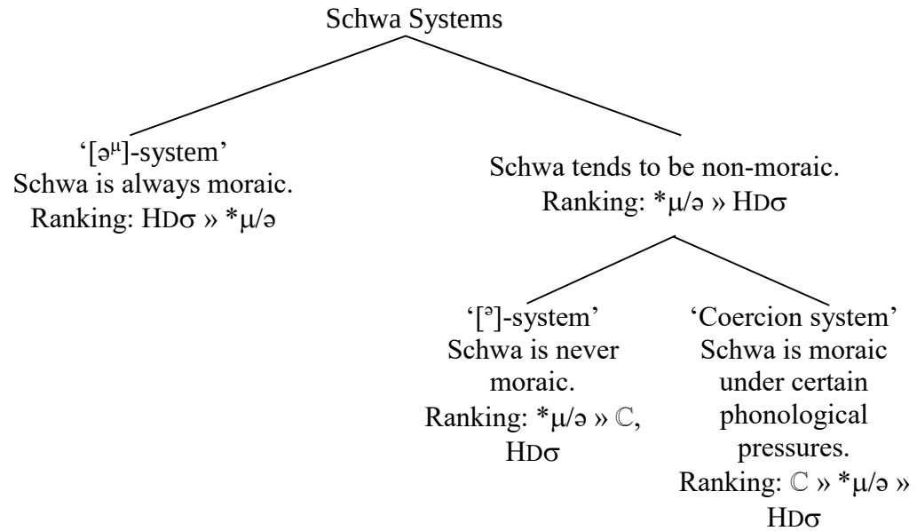
Figure 5.1: Schwa systems.
